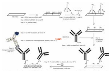
Figure 1. Treatment of a substrate with KOH and O 2 plasma prior to APTES immobilization as part of an APTES-based sandwich ELISA procedure. Reproduced with permission from ref 60. Copyright 2011 Nature America Inc.
