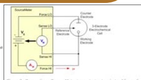
Figure 2. Connecting a Source Meter to an electrochemical cell for cyclic voltammetry
