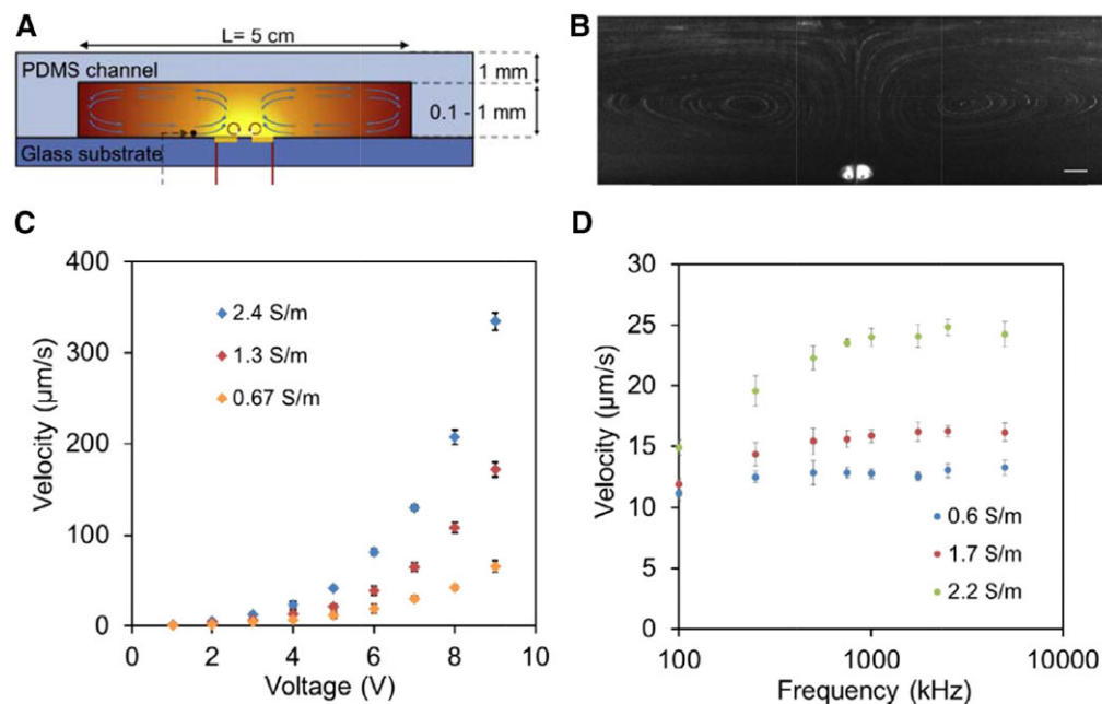
Figure 14. Long-range fluid motion induced by ACET. (A) A cross-sectional view of the microchannel integrated with a pair of parallel electrodes. Arrows indicate the direction of the flow. Black spots represent the location of velocity measurement. (B) Formation of two pairs of counter vortices in the microchannel. Fluorescence images were stacked together to illustrate the trajectories of the microspheres. Performance of the ACEO micropump at different (C) voltage and (D) applied electric field frequency. Reprinted from Lu et al. [41] (2016), with permission from Elsevier.
