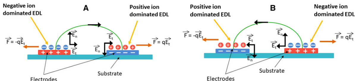
Figure 11. ACEO fluid motion and induced charges at electrode surfaces. (A) During the half cycle when the left electrode has positive polarity and the right electrode has negative polarity; (B) during the next half cycle with opposite electrical polarity. In AC electroosmosis, the bulk electrolyte is electroneutral and behaves in a resistive manner, while the EDL is charged and behave like a capacitor.
