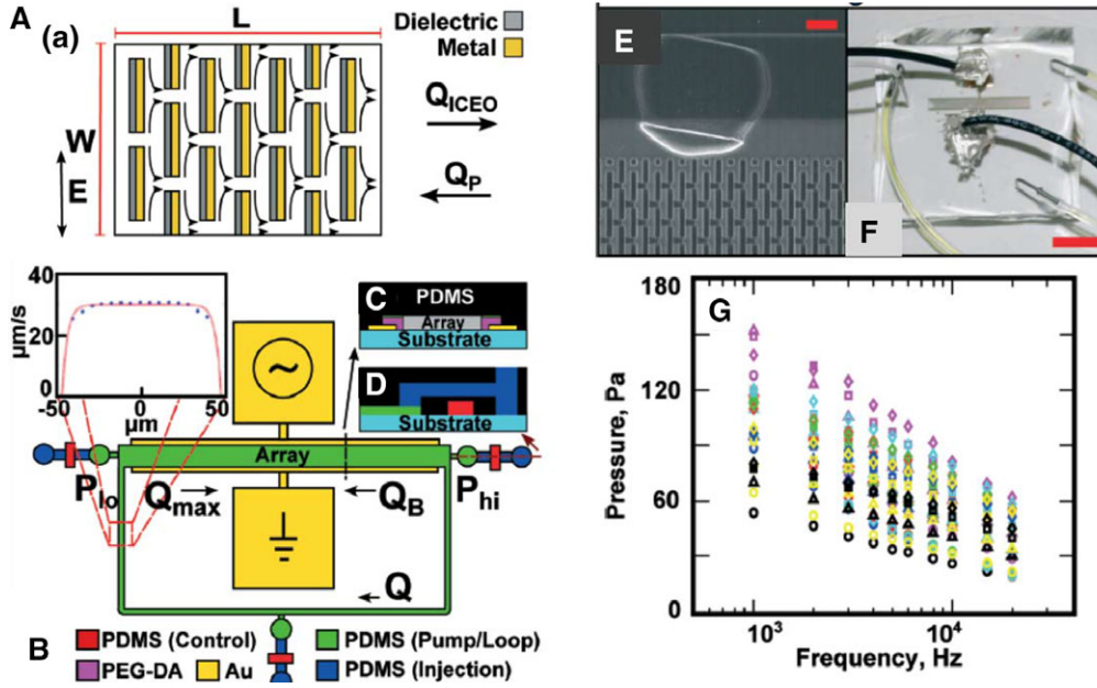
Figure 17. (A) Schematic of ICEO pumping mechanism using an array of metallo-dielectric Janus micro-pillars. The applied AC electric field in vertical direction drives ICEO flow, Q_{ICEO} from left to right. (B) Microfluidic channel for ICEO flow in a loop. The velocity profile was constructed from the microPIV measurement. (C) Side view of array region in the microfluidic ICEO pump. (D) A sectional view of multilayer microchannels at the inlet. (E) SEM image of array region showing electrically permeable hydrogel plugs along the driving electrodes for blocking backflow (scale bar 50 \mu\text{m} ). (F) Picture of a complete working ICEO pumping device (scale bar 1 \text{ cm} ). (G) ICEO pump pressure measured for ten frequencies between 1 and 20 kHz, four different voltages (100 Vpp, circles; 125 Vpp, triangles; 150 Vpp, squares; 175 Vpp, diamonds), and seven electrolytes (KCl, black; NaCl, blue; chloroacetate, pKa 2.9, yellow; acetate, pKa 4.8, cyan; MES, pKa 6.2, green; MOPS, pKa 7.2, red; Tris, pKa 8.3, magenta). Reproduced from Paustian et al. 2014 with permission of the Royal Society of Chemistry.
