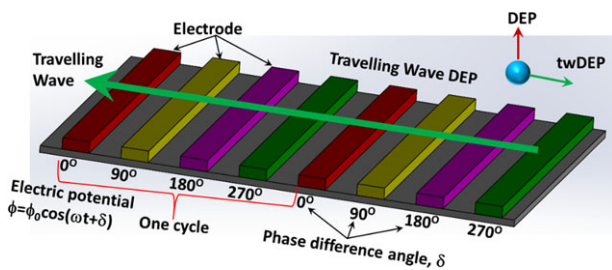
Figure 18. Schematic representation of an array of microelectrodes for traveling wave DEP. Travelling waves are created by using phase difference of \pi/2 between the electrodes. Traveling wave DEP facilitates electrostatic force parallel to the direction of wave propagation in addition to the conventional vertical force. The phase difference creates spatial variation in the electric field which provides a movement of the suspended particles in the fluid media. Hence, it creates unidirectional flow of particles and an induced fluid motions in the microchannel.
