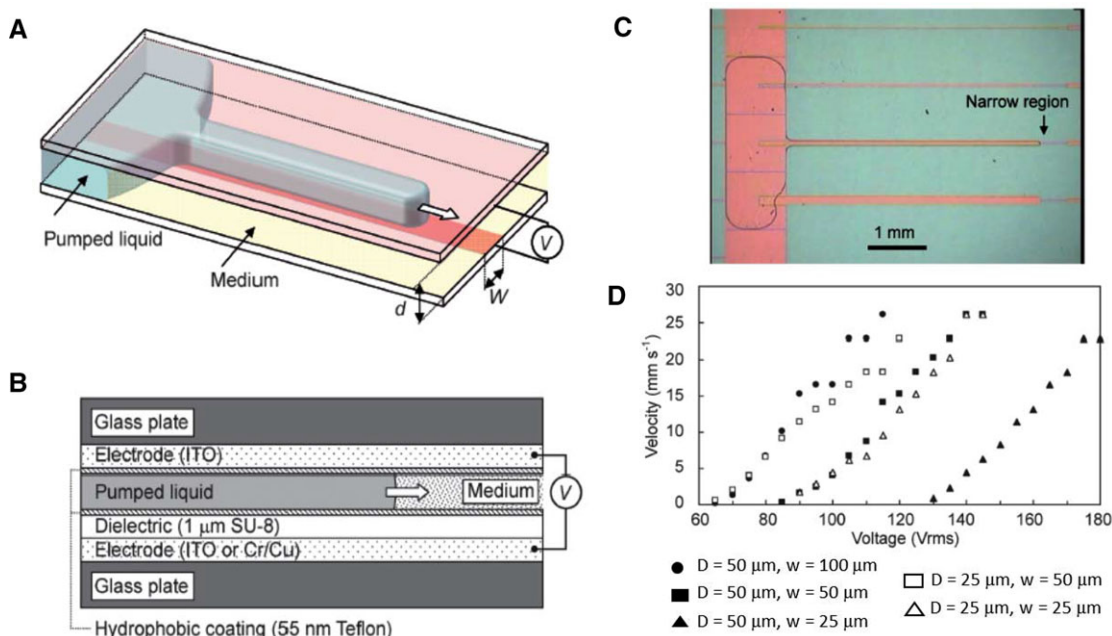
Figure 22. (A) Concept sketching of LDEP pumping mechanism for an electric field defined virtual microchannel. Electric field is applied between unpatterned electrode (top plate) and patterned electrodes (bottom plate) where the channel shape depends on the design of electrode on the bottom plate. (B) Cross-sectional view of device, (C) DI water is flowing over an array of linear electrodes with different width due to the application of 100 kHz AC electric field, and (D) pumping velocity of DI water for various applied electric potentials and aspect ratios i.e. d/w where d is the depth of spacers and w is the width of electrodes. Reproduced from Fan et al. [190] with permission of the Royal Society of Chemistry.
