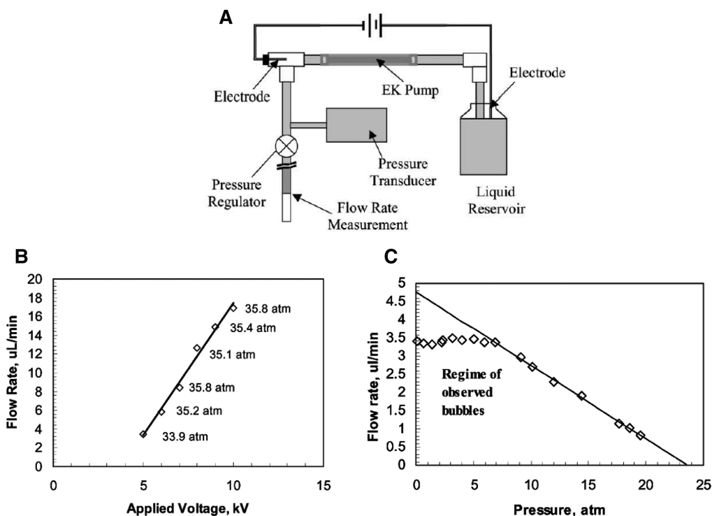
Figure 9. (A) Schematic of the pumping section of a packed column electroosmotic micropump and the test rig to characterize a packed column electroosmotic micropump. The electric field is applied using two platinum electrodes. Pressure transducer and pressure regulator were used to measure the flow rate and the pressure, respectively; (B) Flow rate vs applied voltage at a fixed back pressure; (C) Pump curve (flow rate versus back pressure) for an applied potential difference of 2 kV. The pump's column is 5.4 cm long, 530 \mu\text{m} in diameter, and it is filled with 3.5 \mu\text{m} silica particles. DI water (pH = 5.7, \sigma = 3.0 \mu\text{S}/\text{cm} ) was used as the working fluid in this pump. Reproduced with copyright permissions from Zeng et al. [55].
