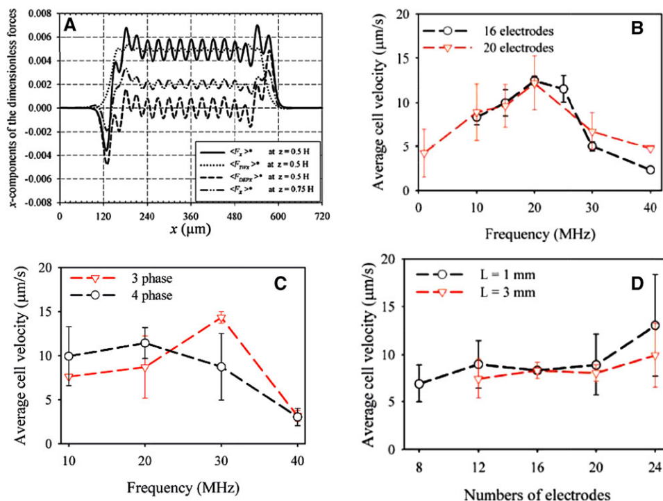
Figure 19. Performance of a traveling wave dielectrophoretic pump for human blood delivery. (A) Distribution of dimensionless conventional DEP and twDEP forces along the channel length. Average cell velocities as a function of (B) applied frequencies, (C) number of phases and (D) number of electrodes. Reproduced from Lei et al. [177] with copyright permission of the Royal Society of Chemistry.
